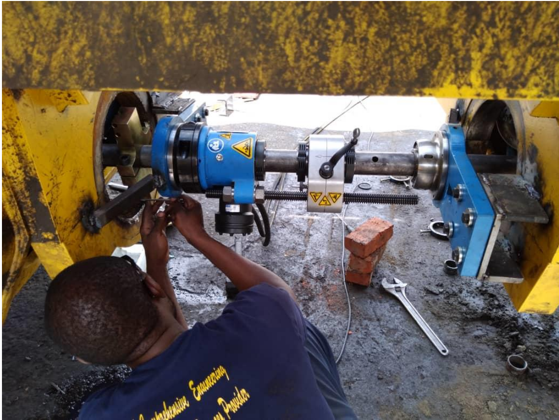
Fig C – Underground Dump Truck Centre Line boring
